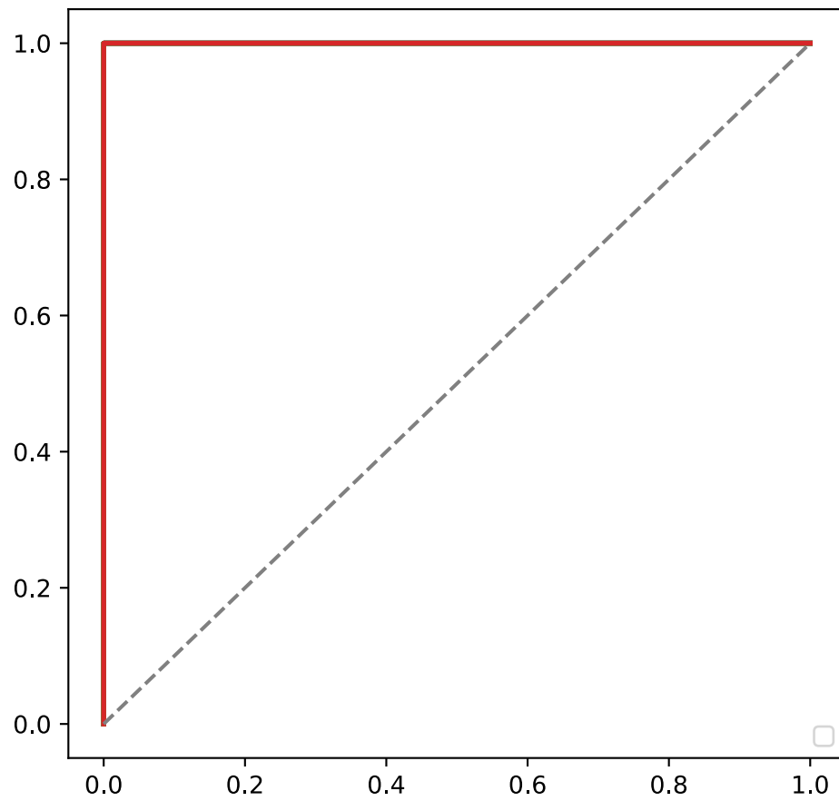
Fold 4
