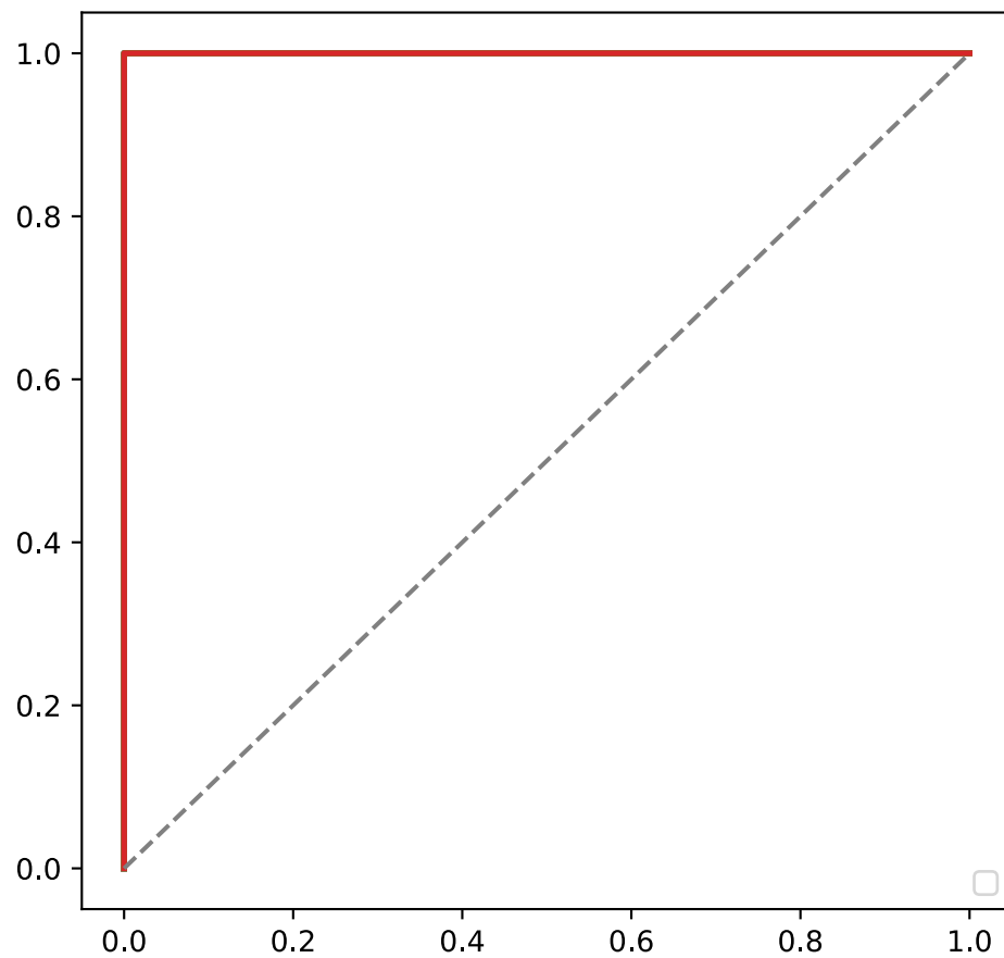
Fold 4
