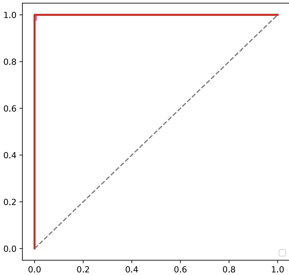
Fold 3
