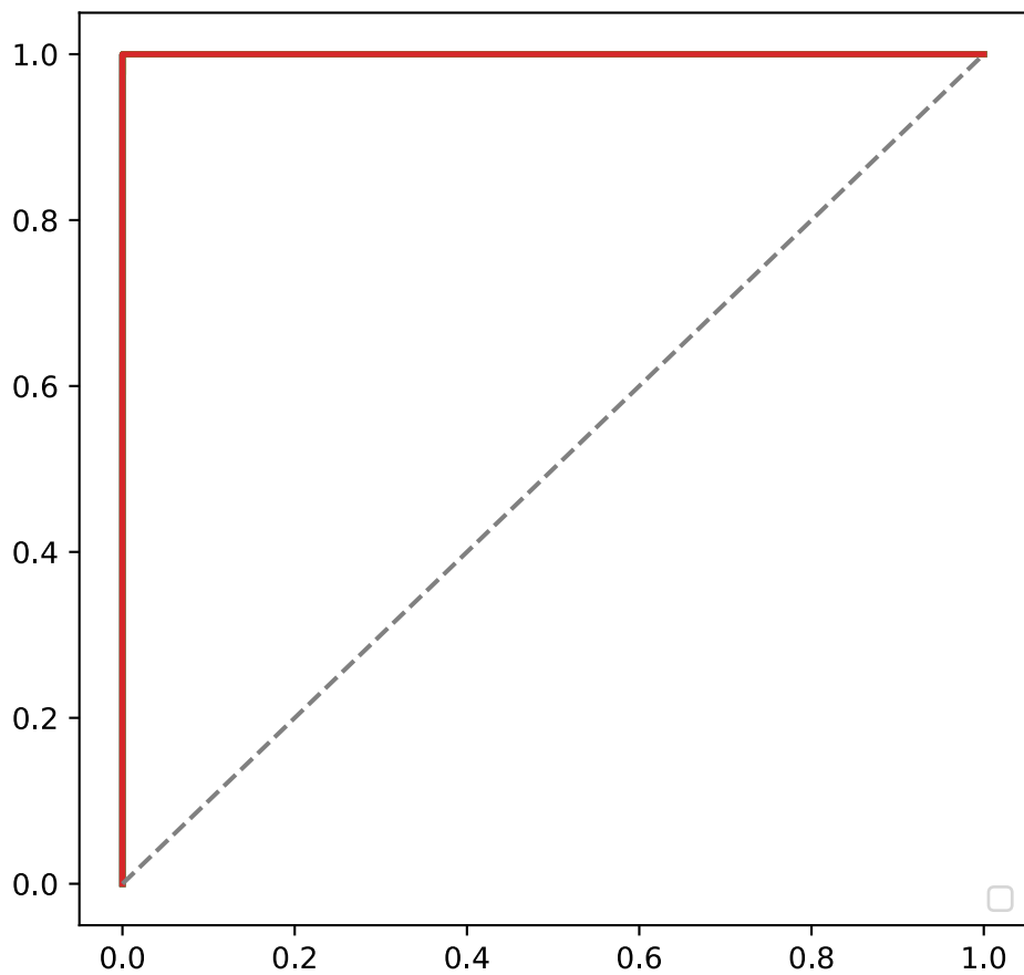
Fold 3
